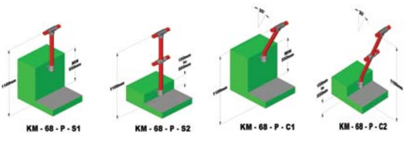
Kee Modules® side fix mounted, handrail tube in-line
