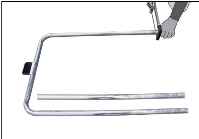
I. Using a hacksaw or similar, carefully cut through the top, bottom tubes and mid rail as shown. For galvanized assemblies, spray with Galvafruid or similar to prevent corrosion.
