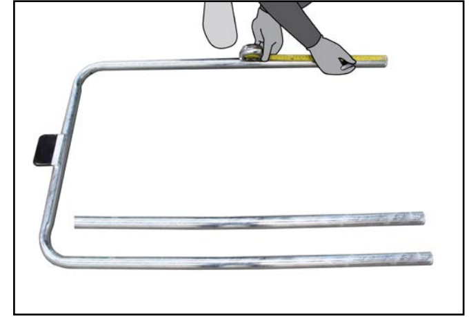
H. Measure the distance recorded in point (f) and mark the gate top and bottom tubes and mid rail as shown.
