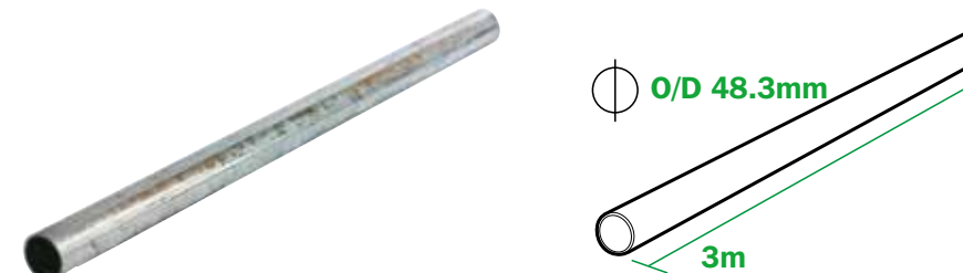
EN 14122-3 SPECIFICATION MAIN RAIL TUBE (3.0m 8-4 AHL) (Cut to size 8-4-AHL-per/m)
