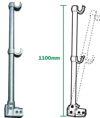
EN 13374 & BS 13700 SPECIFICATION STANDARD SUPPORT LEG - (KGU285)
