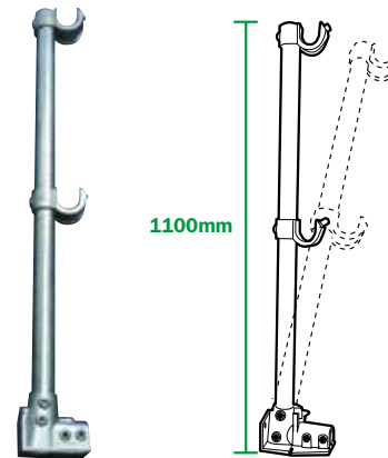
EN 14122-3 SPECIFICATION STANDARD, RAKED, RADIUSED & BENT SUPPORT LEG STANDARD - (KGU45)
