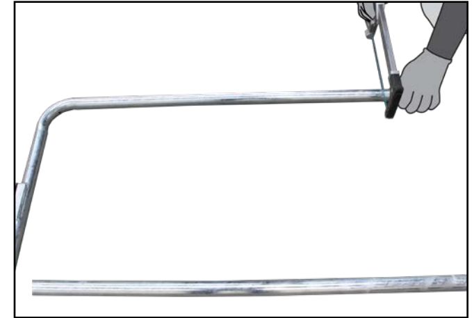
I. Using a hacksaw or similar, carefully cut through the top, bottom tubes, the toeboard and the mid rail as shown. For galvanized assemblies, spray with Galvafroid or similar to prevent corrosion.
