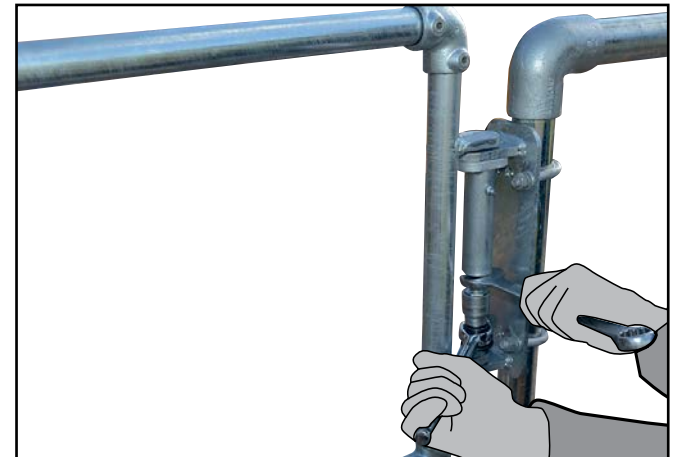
Q. Using the 24mm socket & ring spanner start to tighten the bolt until the gate completely closes. (Note:- You may have to hold the socket whilst using the ratchet).
