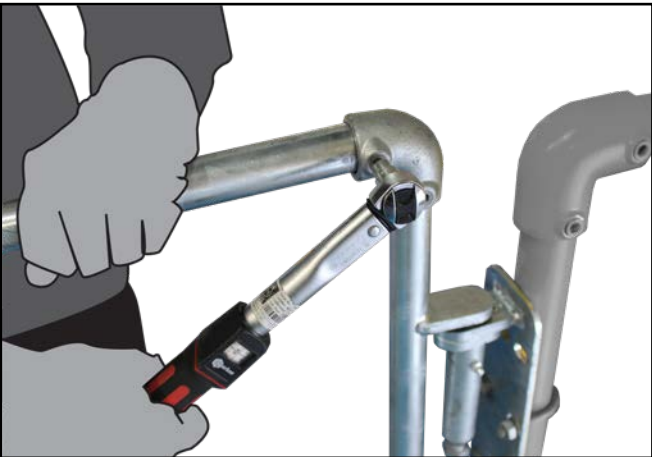
I. Carefully re-position the gate top and bottom tubes into the cast fittings. Ensure the Slam Plate is on the correct side of the Support Leg/Structure. Use a spirit level to ensure the gate is level. Tighten the cast fittings grub screws using a hex head socket. Using the torque wrench ensure the castings are torqued to 39Nm.
