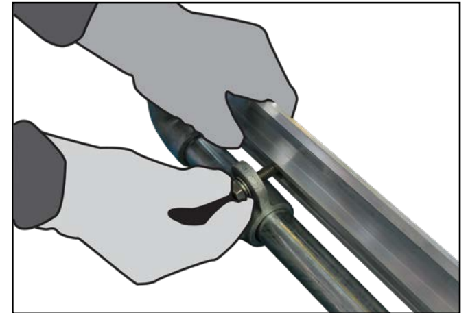
K. Use the supplied M10 nuts, bolts and spring washers to attach the toeboard to the gate.
